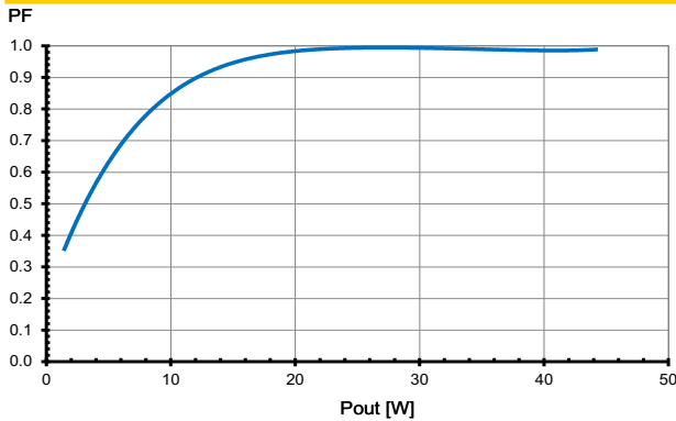
Power factor
