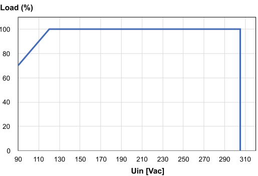
Load (%) vs. Input voltage U_{in} (V AC)
